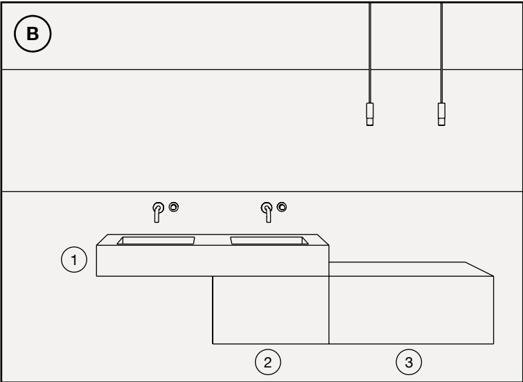
1_DOUBLE FIGURE 121,7 Lavabo integrato doppia vasca Integrated top with two washbasins 2_FRAME 61,7 Mobile sottolavabo Washbasin vanity unit 3_FRAME 86,7 Mobile sottolavabo Washbasin vanity unit
