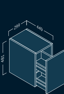
MODULE DOUBLE DRAWER
