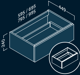
MODULE 1 DRAWER WITHOUT SIPHON SAVER OR ORGANIZER
