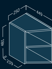
MODULE CHAMFER REVERSIBLE | DEPTH 45 TO 24
