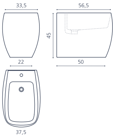
Flò floor-mounted bidet
