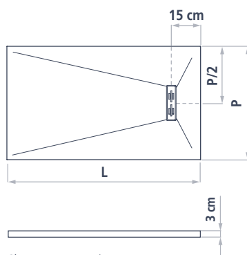
Shower tray section average slope: 1,8%
