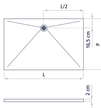
Shower tray section average slope: 2%
