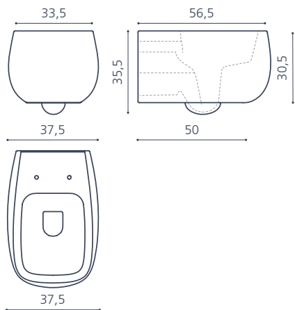
Flò suspended wc
