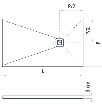
Shower tray section average slope: 1,8%
