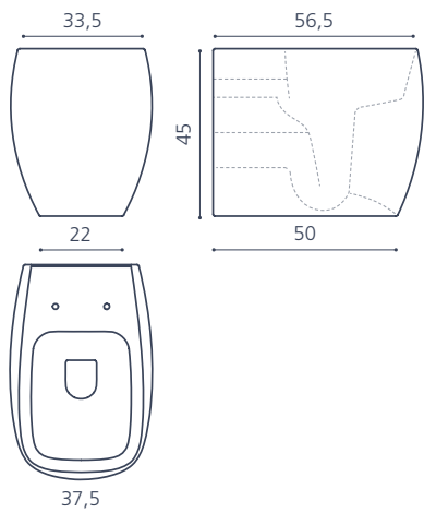
Flò floor-mounted wc
