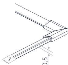
Threshold bar system
