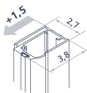
Closing side configuration in niche
