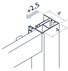
Closing side configuration niche 1 sliding door, saloon folding door and wing door
