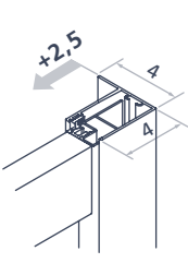
Configuration niche 1 sliding door and 2 central sliding doors
