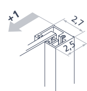
Fixed side and Plus door side, sliding door and asymmetric door
