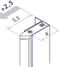
Closing side configuration in niche
