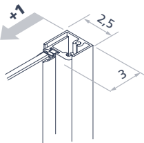
Closing side configuration in niche
