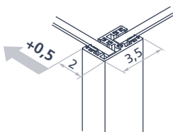
Corner to wall configuration
