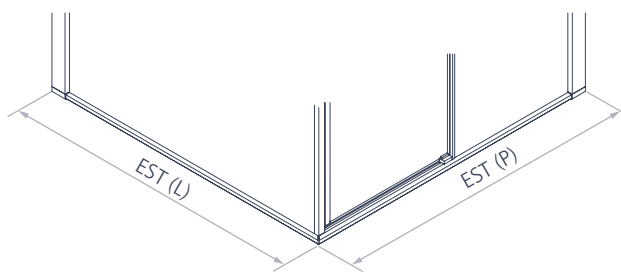
Example with 1 sliding door + 1 fixed side
