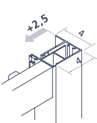
Closing side configuration niche 1 sliding door
