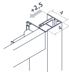
Closing side configuration niche 2 sliding doors
