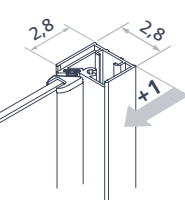
Closing side niche configuration
