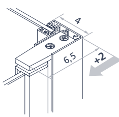
Additional side combined to door side
