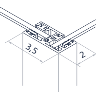
Corner configuration asymmetric
