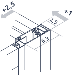
Above wall
