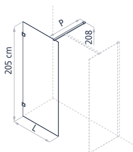
Frontal fixed side
