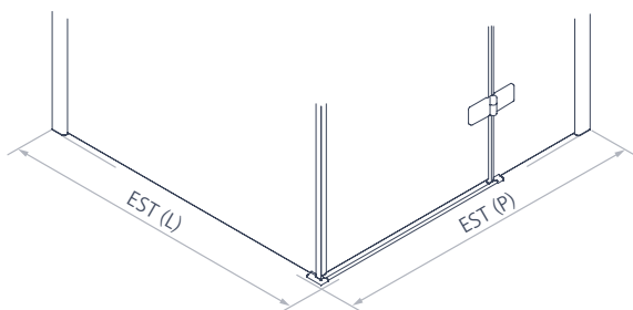
Example with 1 wing door + 1 fixed side
