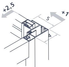
Additional side
