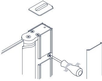
Folding door
