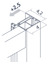
Closing side configuration niche door and round door, 1 sliding door
