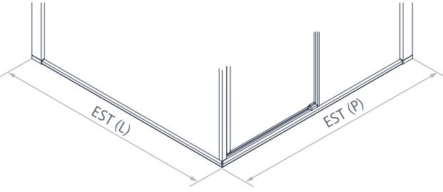
Example with 1 sliding door + 1 fixed side
