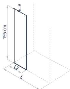
Fixed side (01)
