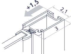
Closing side niche configuration
