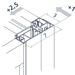
Above wall
