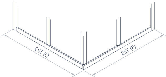
Example with 2 sliding doors
