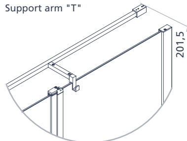
Support arm "T"
