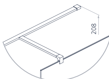
"T" configuration of the "S" support arm
