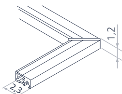
Lower Profile
