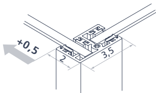
Corner to wall configuration
