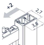
Wing door side
