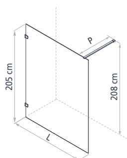
Fixed side
