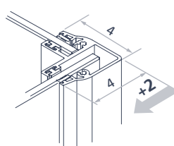
Additional side combined to fixed side
