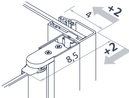
Corner version combined to door side
