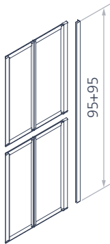
Overlapping doors side
