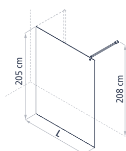
Frontal fixed side
