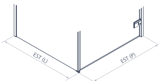
Example with 1 wing door + 1 fixed side
