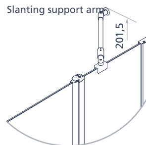
Slanting support arm
