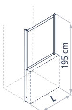
Additional side (02)
