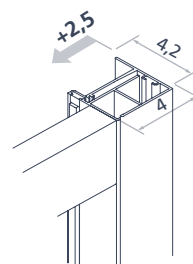
Closing side configuration niche 2 folding doors, 2 saloon doors, 1 wing door
