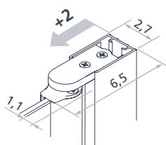
Closing side configuration in niche
