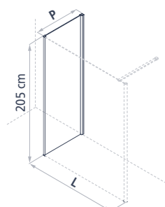
Lateral fixed side
