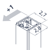
Closing side configuration in niche, wing door, Plus and folding door
