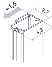
Closing side configuration in niche
