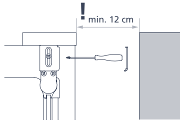
To allow adjustment, consider the indicated distance
