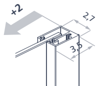
Fixed side and Plus door side, sliding door and asymmetric door
