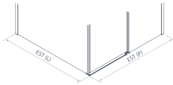
Example with 1 sliding door + 1 fixed side
