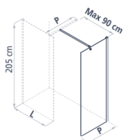
Lateral fixed side
