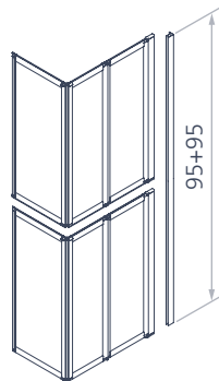
Overlapping doors side for wall configuration
