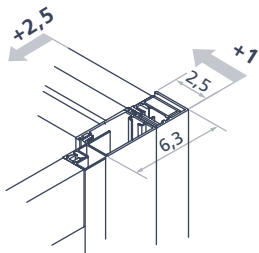
Above wall
