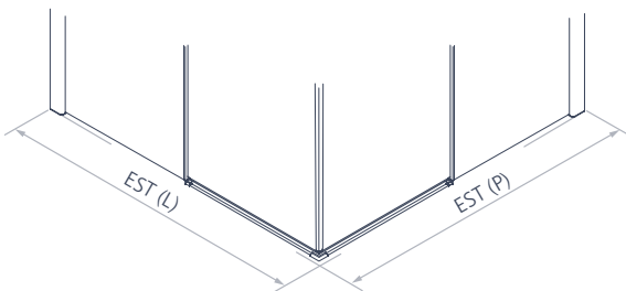
Example with 2 sliding doors
