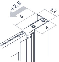
Folding door
