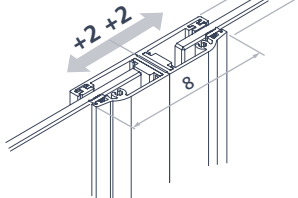
Aligned version combined to fixed side
