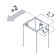
Closing side configuration in niche, sliding door
