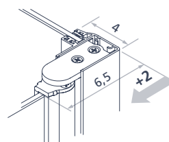
Additional side combined to door side
