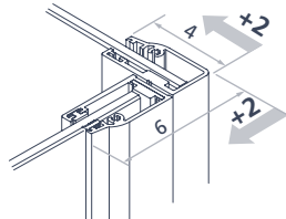
Corner version combined to fixed side
