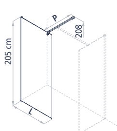
Frontal fixed side
