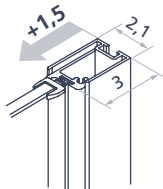
Closing side niche configuration
