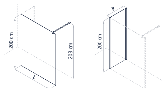
Frontal fixed side
