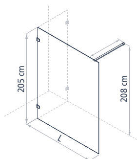
Frontal fixed side
