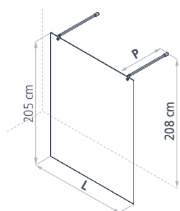
Fixed side
