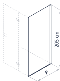
Fixed side combined to glass fixed side (00)
