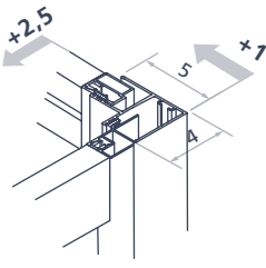
Additional side
