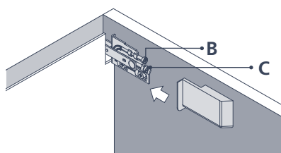
Hanger for storage unit and columns
