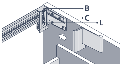
Hanger for basin unit
